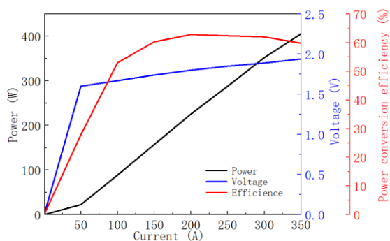
Power-Current-Voltage-Efficiency
